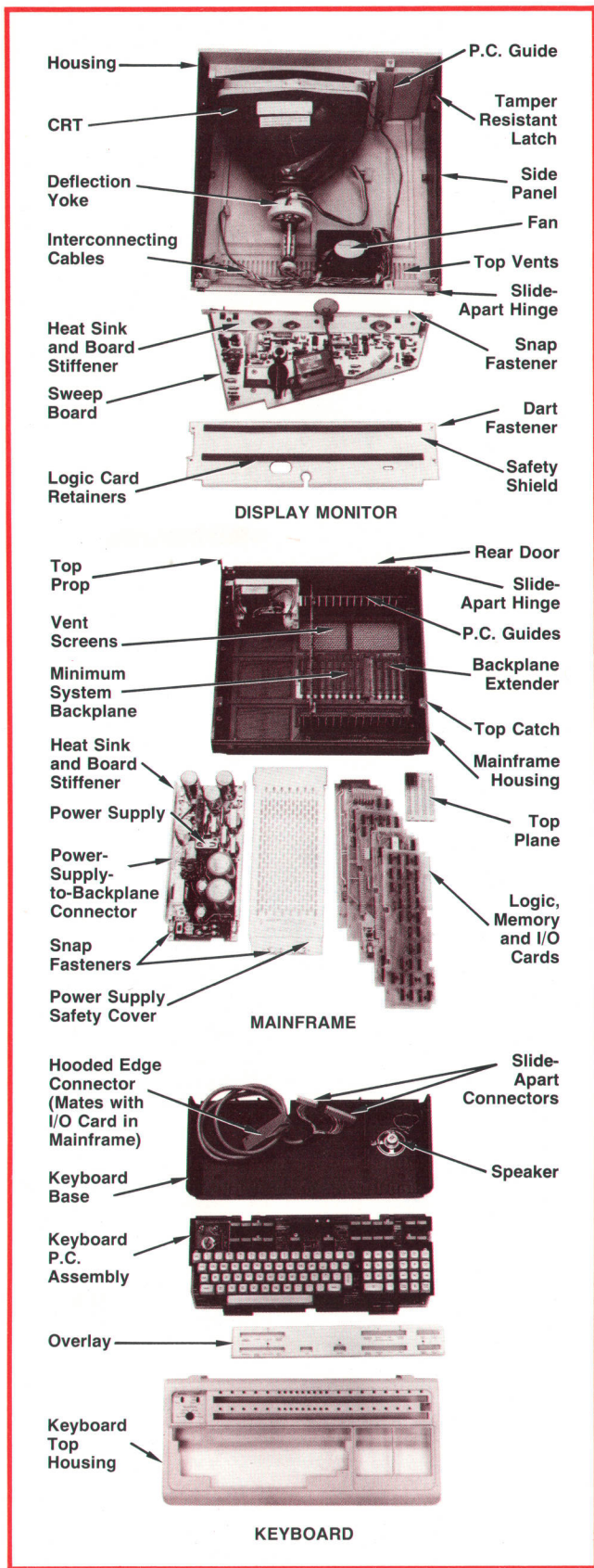
Fig. 1. The 2640A Terminal is designed with pop in/pop-out modularity. The only tool required to replace a module is a key to get inside. Any module can be replaced in two minutes.
