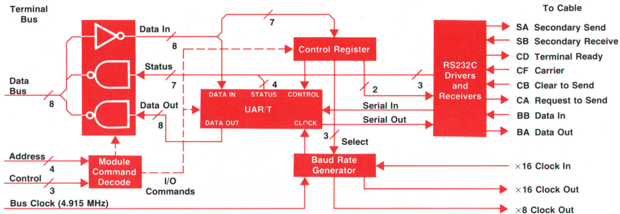
Data communications module.
