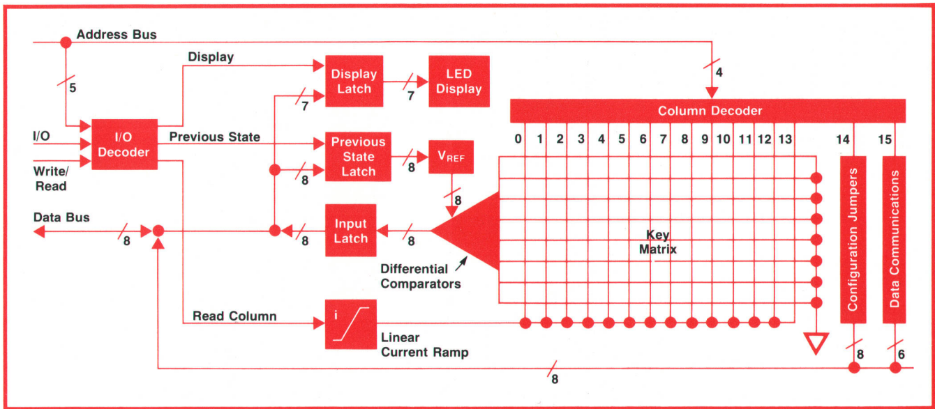
Fig. 2. Keyboard hardware implementation. Each key is assigned a position in a matrix of sixteen columns and eight rows. The microprocessor scans this matrix continuously, reading one column at a time.
