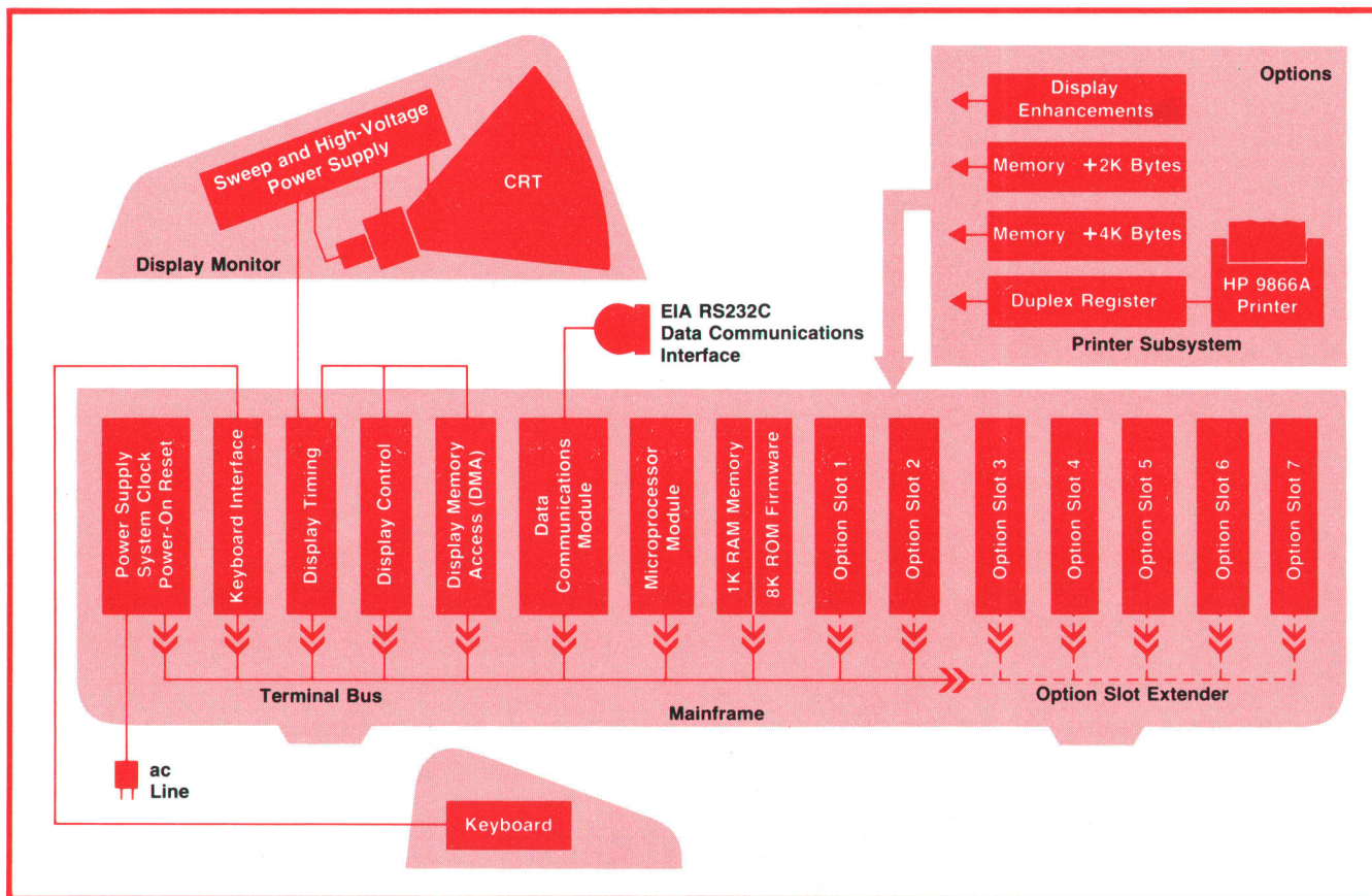
Fig. 2. CRT monitor, mainframe, and keyboard form three mechanically independent sections. Mainframe contains slots for standard and optional modules. Any module, including the power supply, can be replaced quickly without tools.
